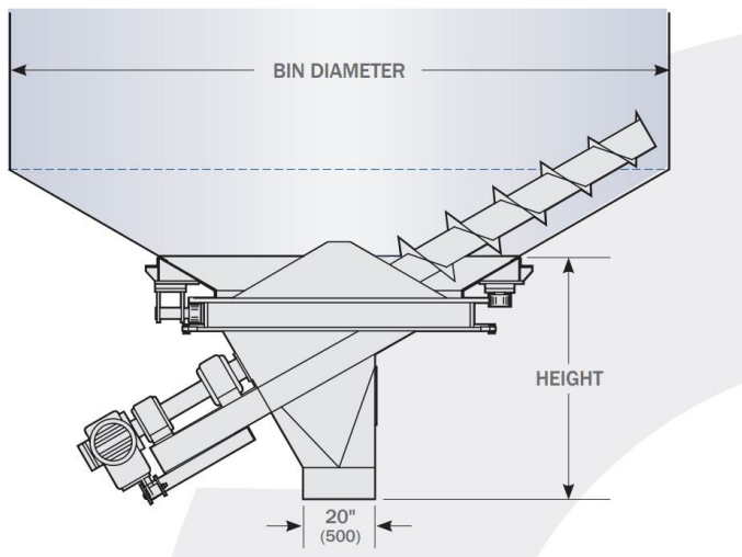
APPROXIMATE LAYOUT DIMENSIONS* AND SHIPPING WEIGHTS FT. (M)
