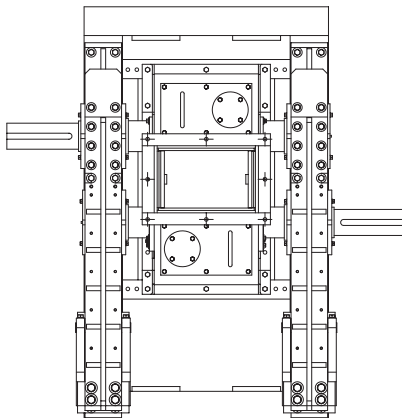
FRONT OF CRUSHER
