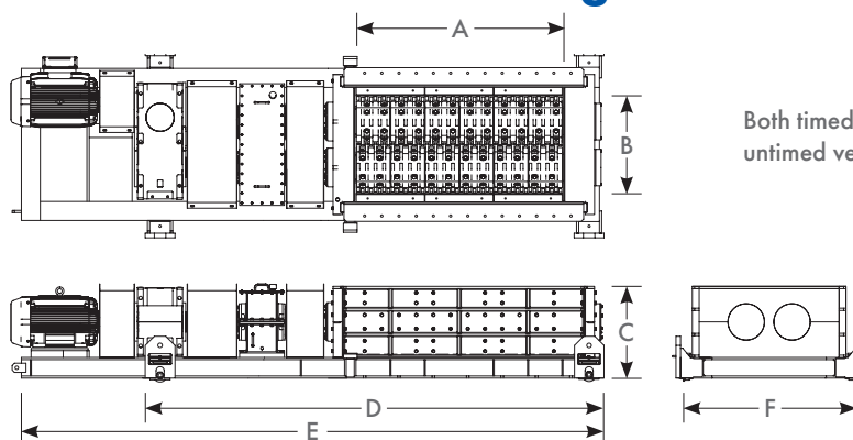
APPROXIMATE LAYOUT DIMENSIONS AND SHIPPING WEIGHTS IN (MM)
